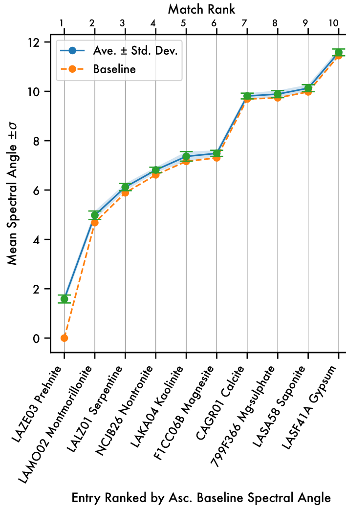
LAZE03 Prehnite Mean Spectral Angle Match
